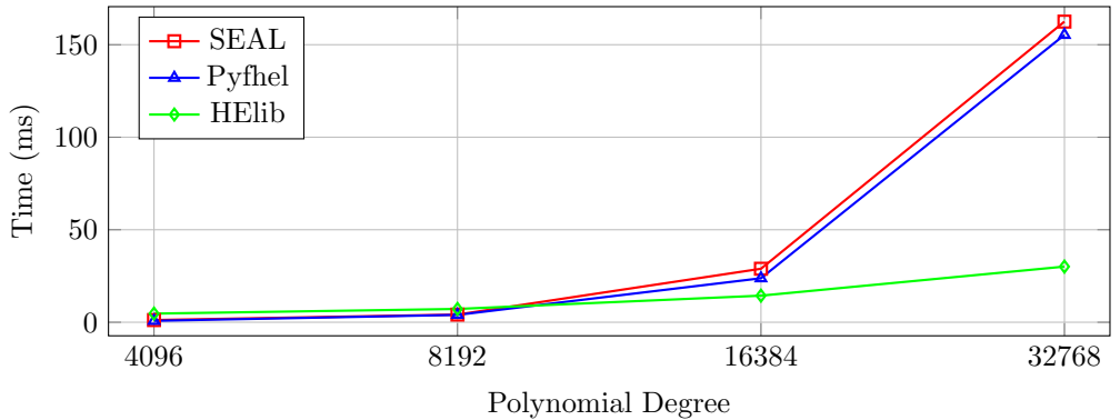
Figure 1: Comparison of rotation operation performance across libraries (SEAL and Pyfhel without HEXL, HELib with HEXL as reference)
